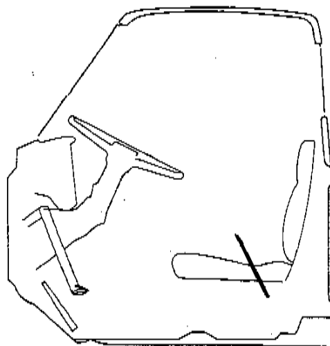
FIG. 1—TRUCK ACCOMMODATION TOOL REFERENCE LINE
