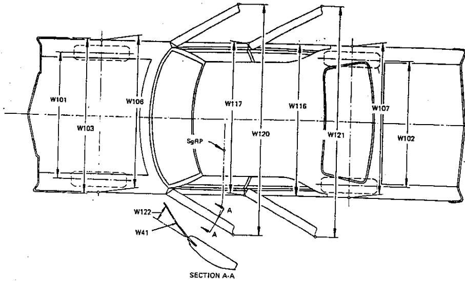
FIG. 18—EXTERIOR DIMENSIONS, WIDTH
