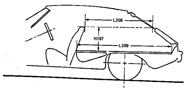
φFIG. 28—CARGO SPACE DIMENSIONS, HATCH BACK
