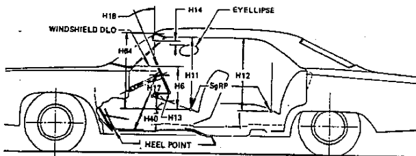
FIG. 8—INTERIOR DIMENSIONS, HEIGHT
