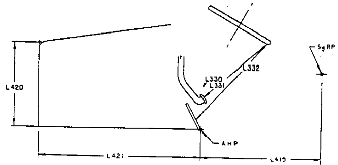
φFIG. 17—PEDALS TO STEERING WHEEL CLEARANCE
