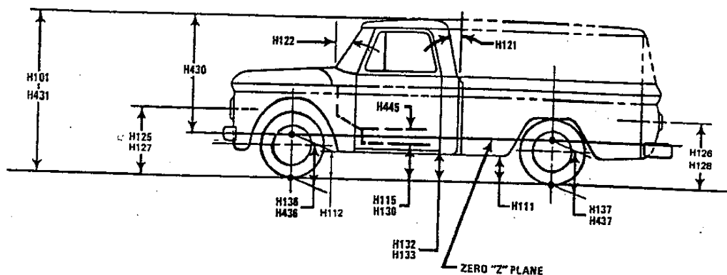
φFIG. 22—EXTERIOR DIMENSIONS, HEIGHT—TRUCK
