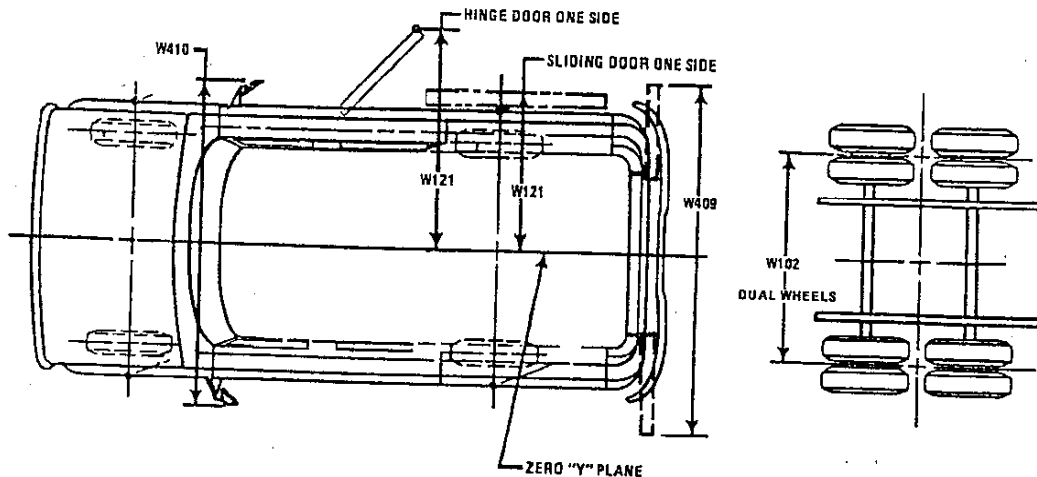
FIG. 19—EXTERIOR DIMENSIONS, WIDTH—TRUCK
