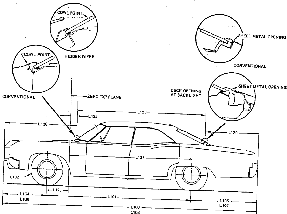
φFIG. 23—EXTERIOR DIMENSIONS, LENGTH
