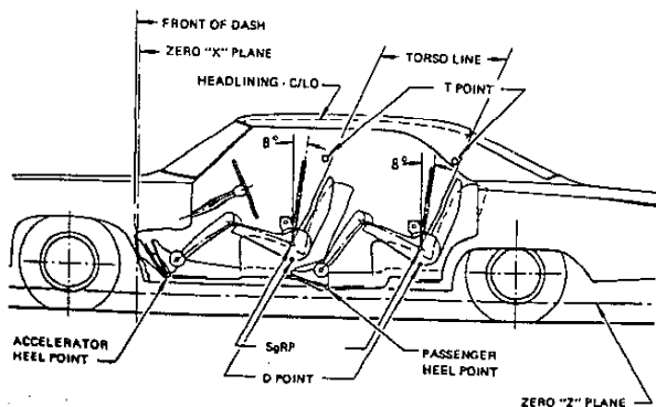
FIG. 1—REFERENCE POINTS
