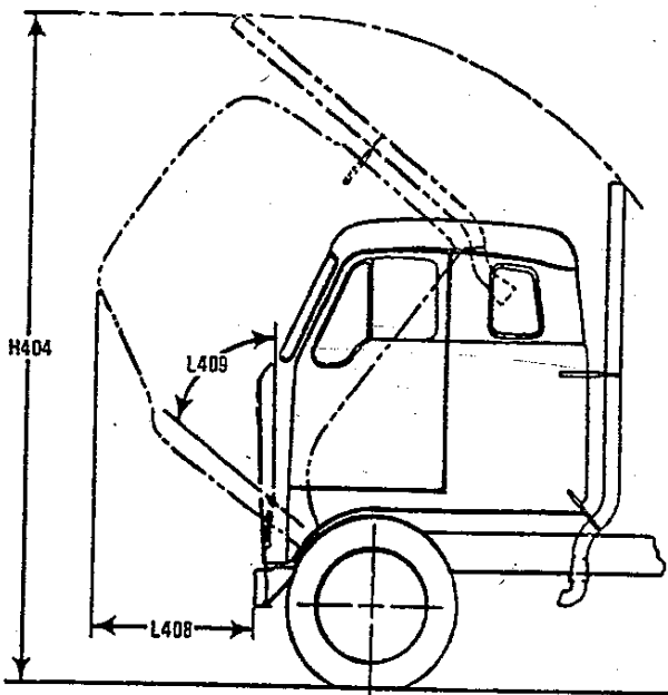
φFIG. 25—CAB SERVICING DIMENSIONS
