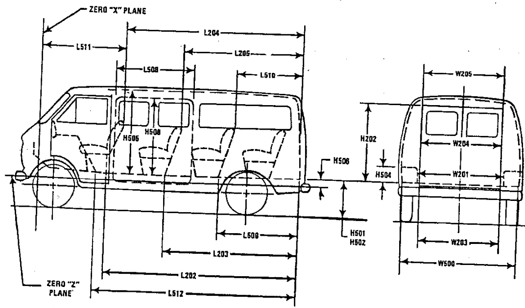
φFIG. 29—CARGO SPACE DIMENSIONS, TRUCK AND MPV WITH CLOSED CARGO AREA
