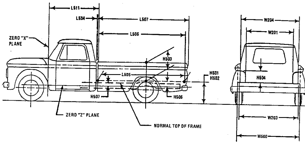
φFIG. 30—CARGO SPACE DIMENSIONS, TRUCK WITH OPEN CARGO AREA
