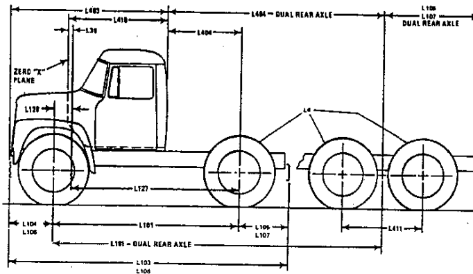
φFIG. 24—EXTERIOR DIMENSIONS, LENGTH—TRUCK
