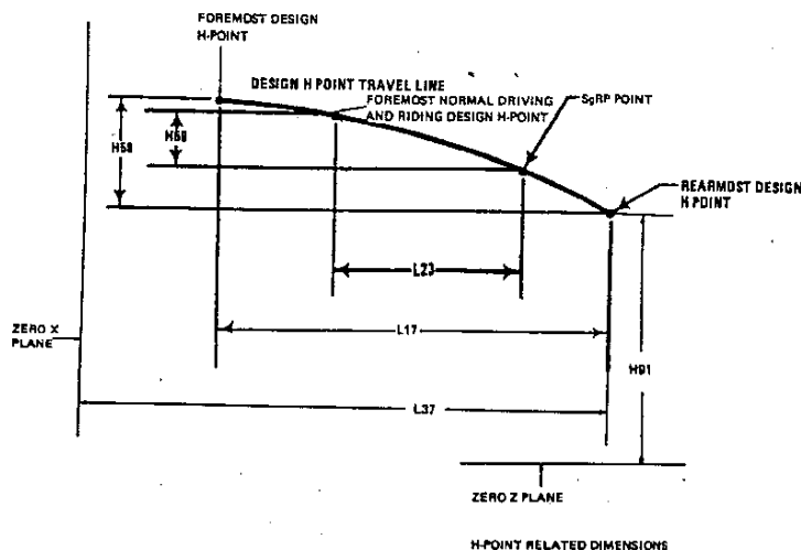
FIG. 9—H-POINT RELATED DIMENSIONS
