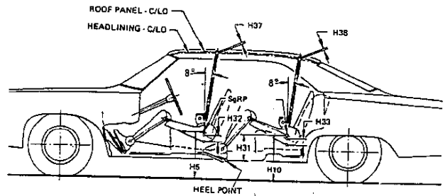
φFIG. 3—INTERIOR DIMENSIONS, HEIGHT
