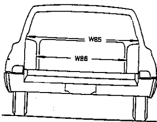
FIG. 16—INTERIOR DIMENSIONS, STATION WAGON THIRD SEAT
