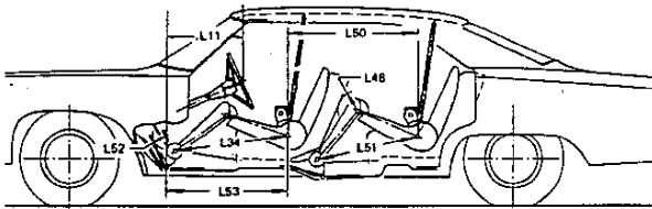
φFIG. 12—INTERIOR DIMENSIONS, LENGTH
