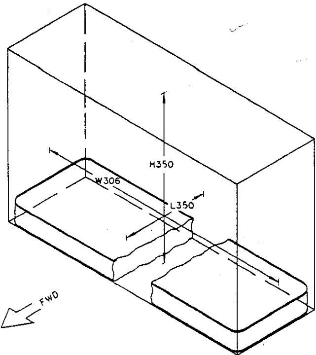
φFIG. 15—TRUCK SLEEPER COMPARTMENT
