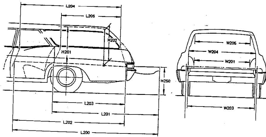
φFIG. 27—CARGO SPACE DIMENSIONS, STATION WAGON
