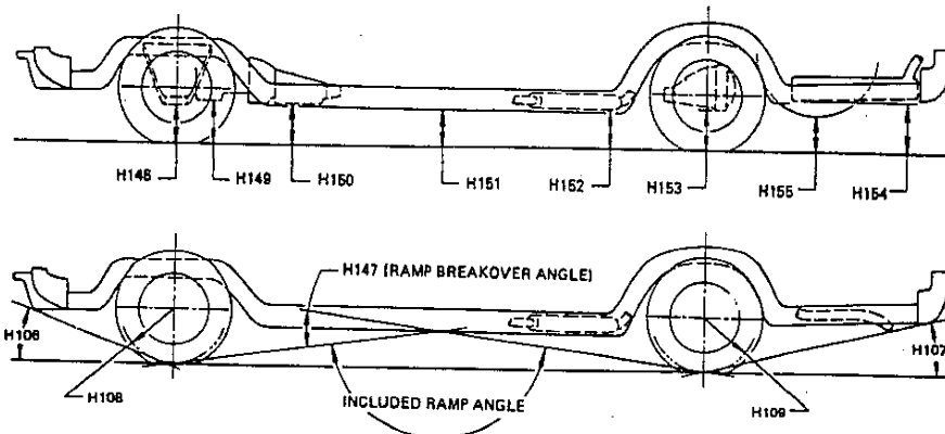
φFIG. 26—GROUND CLEARANCE DIMENSIONS
