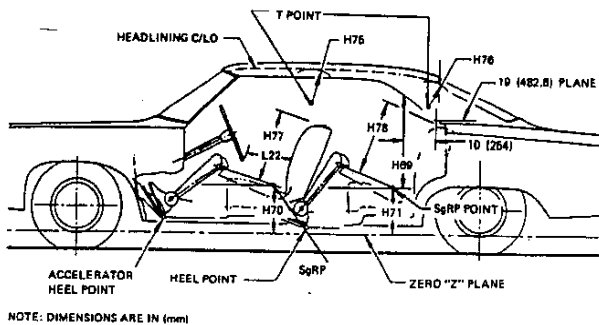
FIG. 7—INTERIOR DIMENSIONS, HEIGHT
