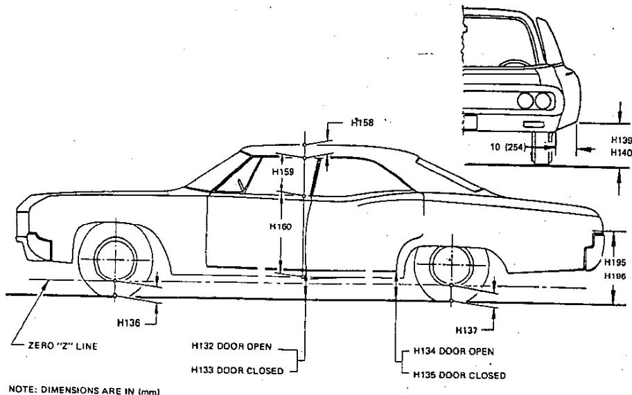
φFIG. 21—EXTERIOR DIMENSIONS, HEIGHT
