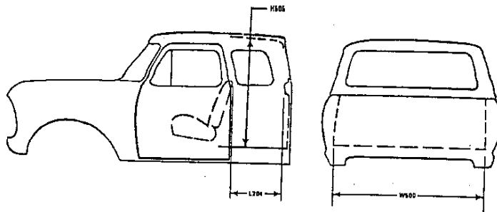
φFIG. 31—CARGO SPACE DIMENSIONS, TRUCK WITH CLOSED CARGO AREA
