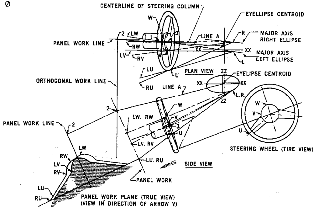
FIG. 15—DRAFTING PROCEDURE FOR CONSTRUCTING THE OBSCURED AREA CAUSED BY THE STEERING WHEEL HUB AND HORIZONTAL SPOKES
