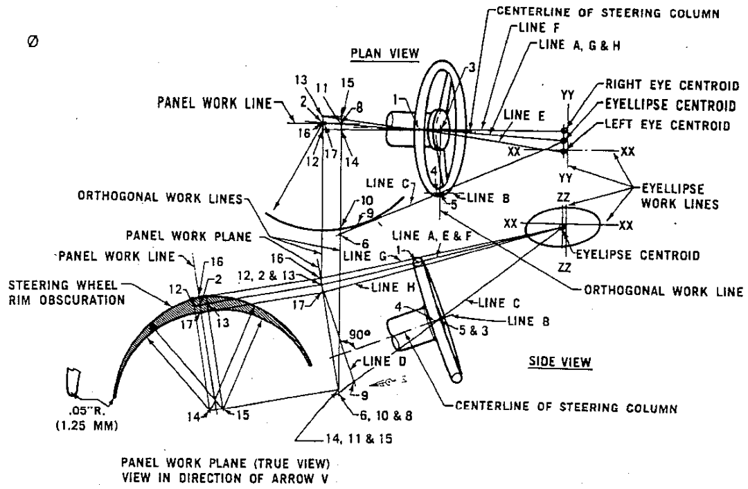
FIG. 13—DRAFTING PROCEDURE FOR CONSTRUCTION—THE STEERING WHEEL RIM OBSCURATION
