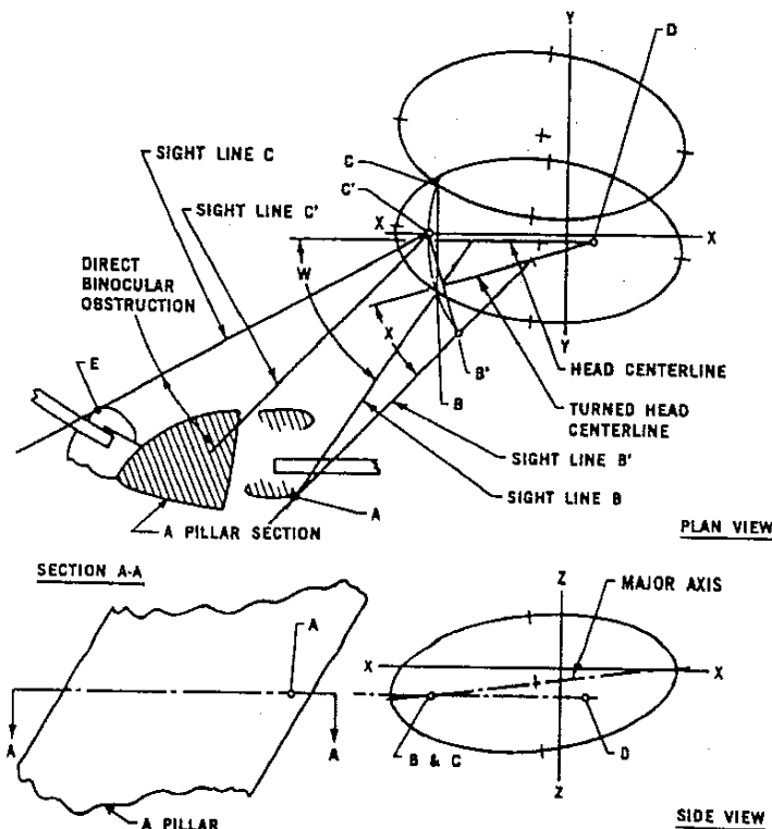
FIG. 9—DIRECT BINOCULAR OBSTRUCTION
