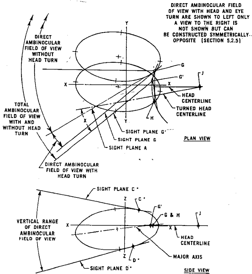
FIG. 8—DIRECT AMBINOCULAR FIELD OF VIEW (EYE AND HEAD MOVEMENT)
