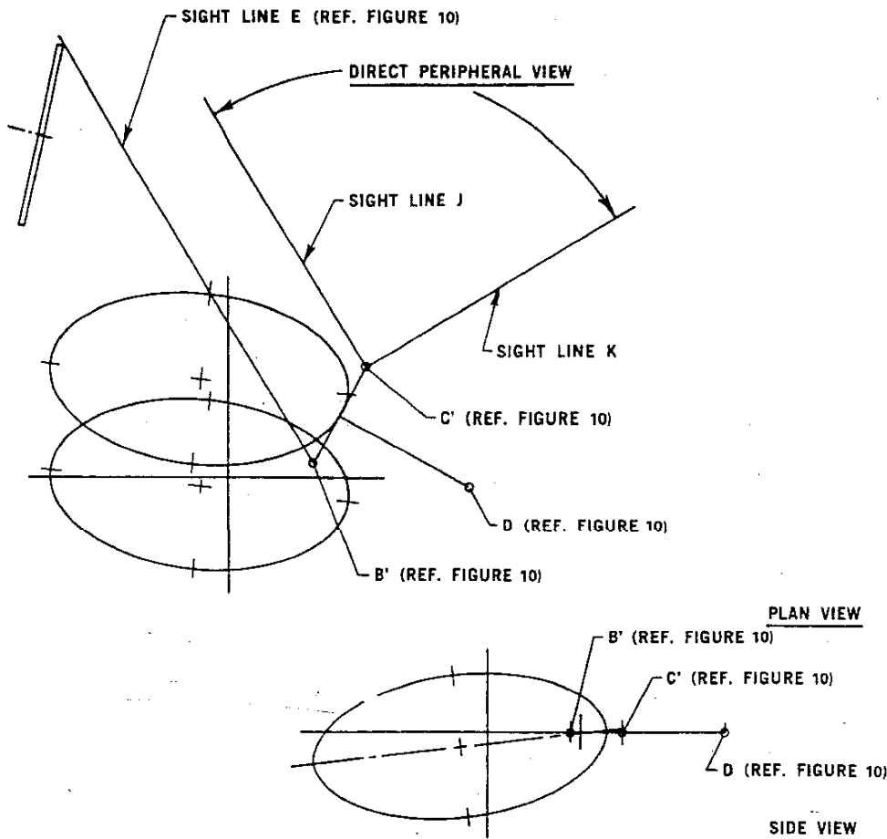
FIG. 12—DIRECT PERIPHERAL VIEW
