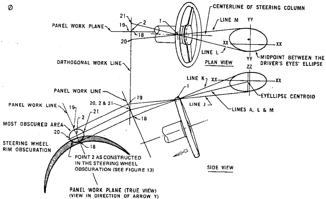
FIG. 14—DRAFTING PROCEDURE FOR SCANNING THE PANEL WORK PLANE WITH THE STEERING WHEEL RIM OBSTRUCTION
