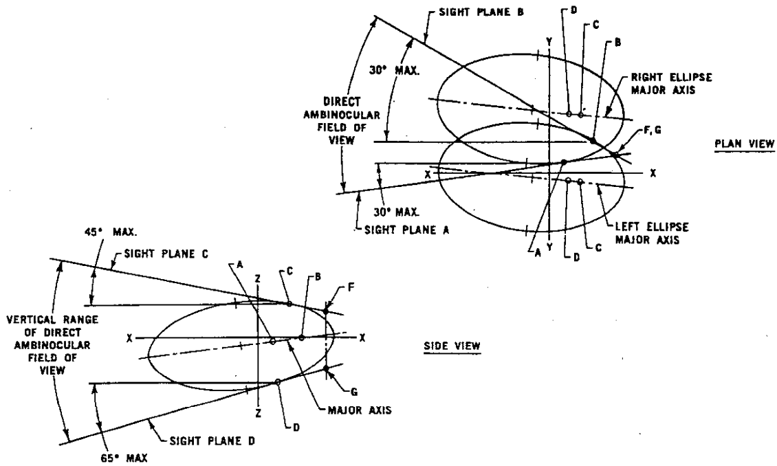
FIG. 7—DIRECT AMBINOCULAR FIELD OF VIEW (EYE MOVEMENT ONLY)
