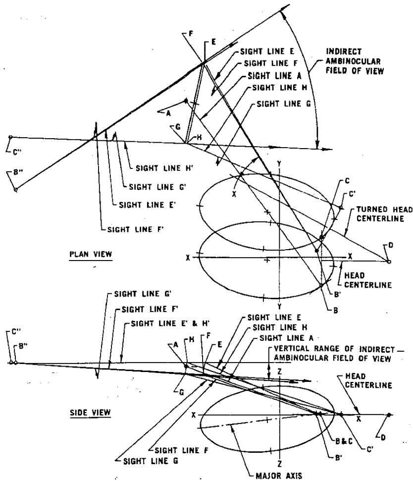
FIG. 10—INDIRECT—AMBINOCULAR FIELD OF VIEW
