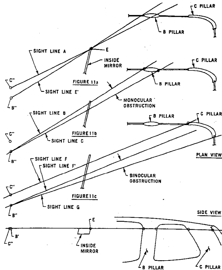
FIG. 11—INDIRECT—MONOCULAR AND BINOCULAR OBSTRUCTIONS
